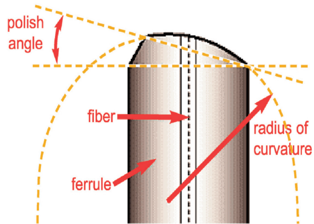
4.0 ANGLED POLISH The end face is polished at an angle relative to the axis perpendicular to the ferrule axis.
