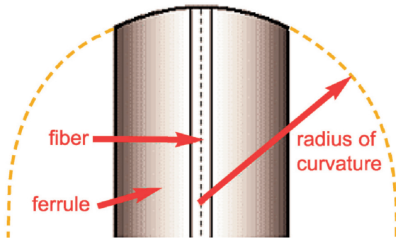
1.0 POLISH RADIUS The radius of curvature is defined as the radius of the end-face surface as measured from the ferrule axis.
