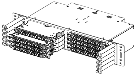
Optical Component Chassis (4")
