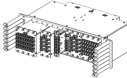
Optical Component Chassis LGX Style (6")
