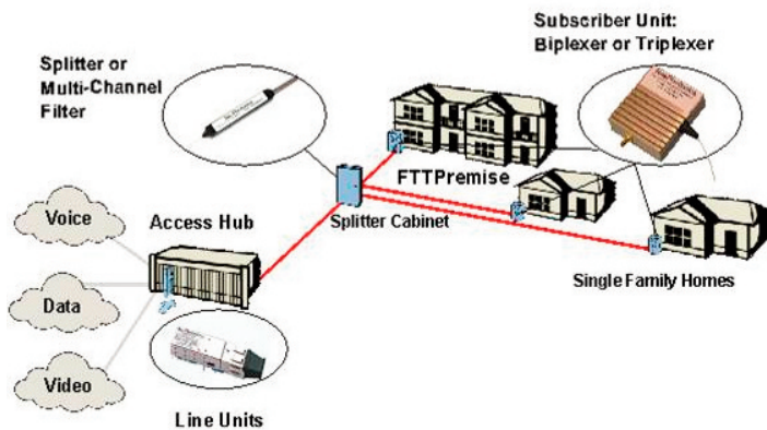
Passive Optical Network Architecture
